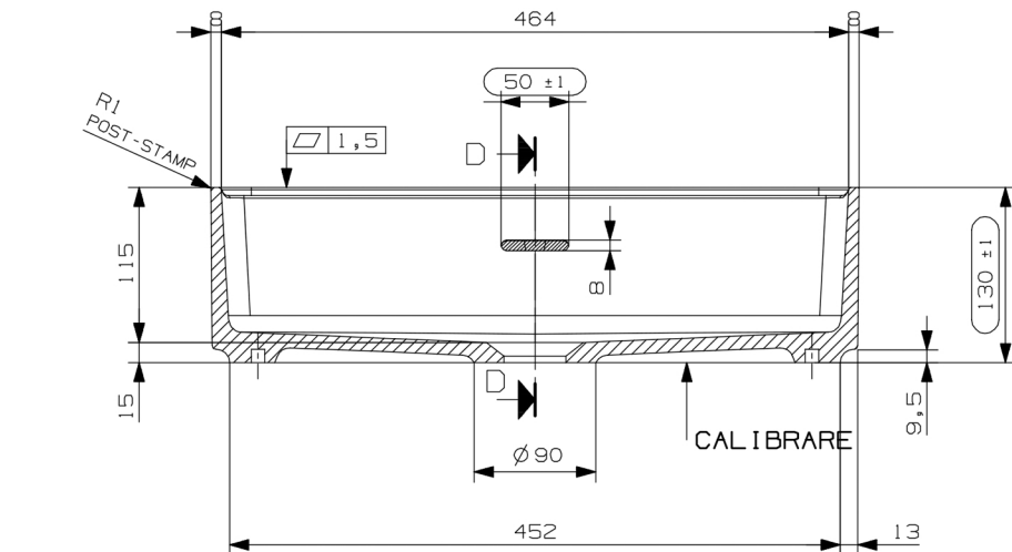
SECTION C-C SCALE 1:4
